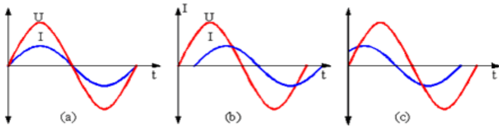
a- resistive power b- inductive power c- capacitive power
